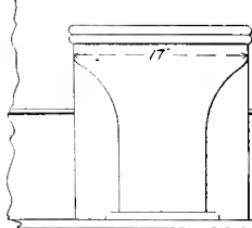
Figs. 3857-3859. THE "STANDARD" DRY-CLOSET HOPPER AND SEAT. HENRY C. HART MANUFACTURING COMPANY.
